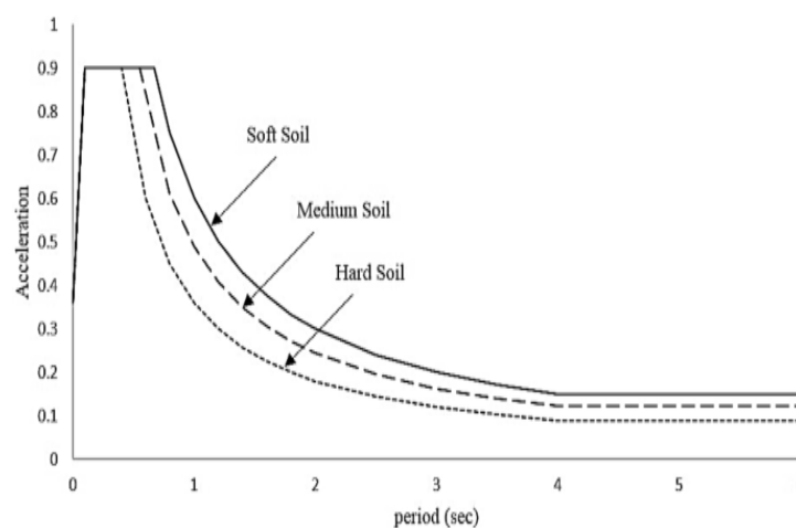
Fig. 1: Curvature between Acceleration vs. Time period of hard, medium and soft soil.
